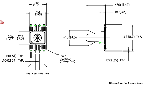
Single Pressure Port Dual in Line BARO-AF-PRIME-DIP
