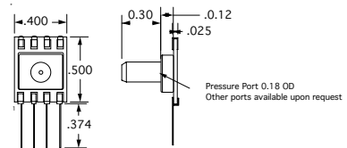
Single Pressure Port BARO-AF-PRIME-MINI
